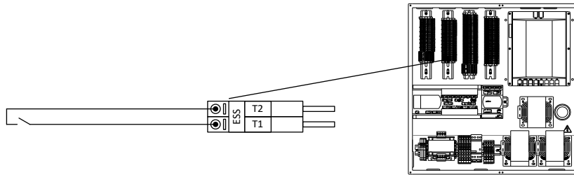
Figure 5.11. Connection scheme of the external protection devices
