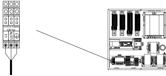
Figure 5.8. Connection scheme of the NETZERO heat pump control power supply.
